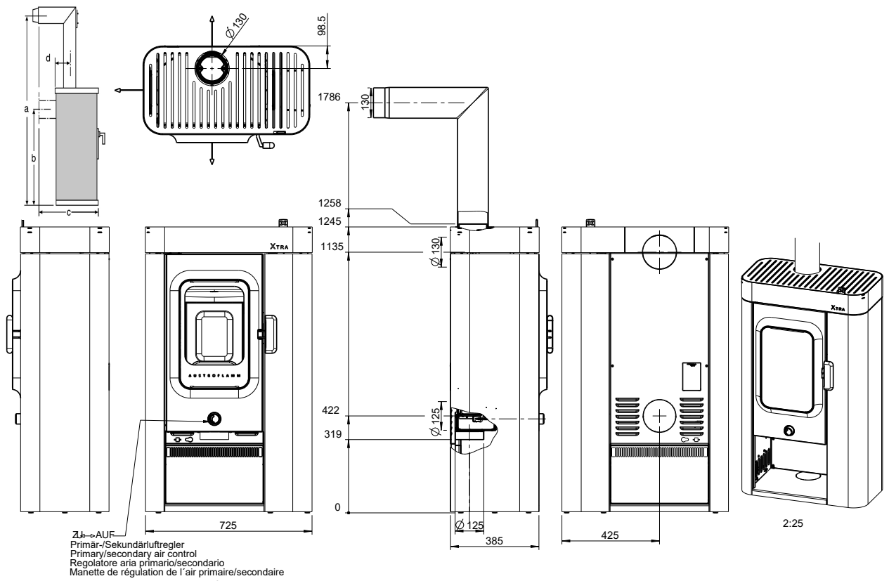
Fig. 2: Dimensions, Xtra incl. (option)
